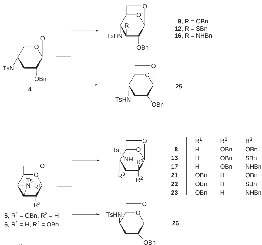
SCHEME 3
